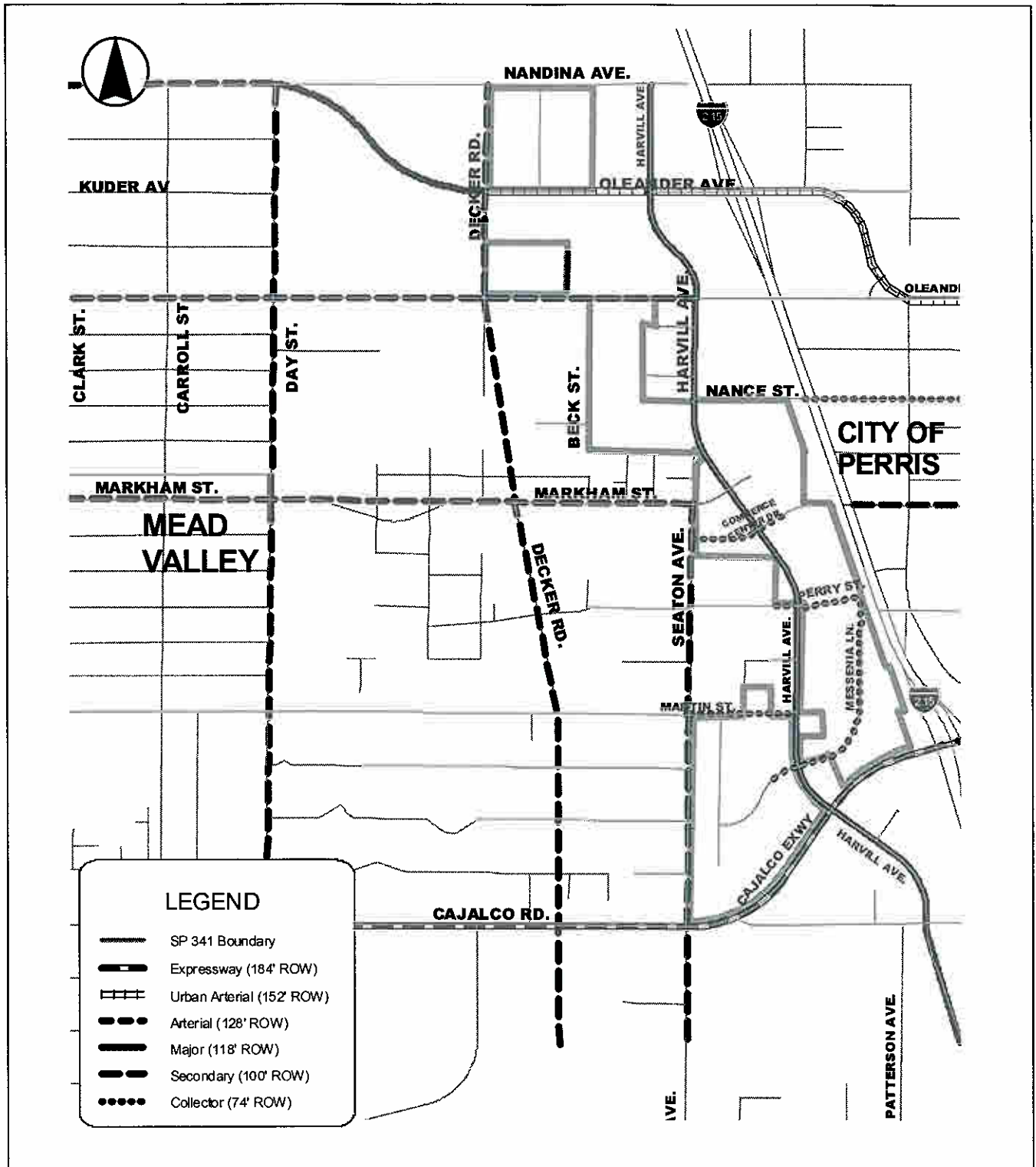
Figure III-4 Circulation Plan Majestic Freeway Business Center
